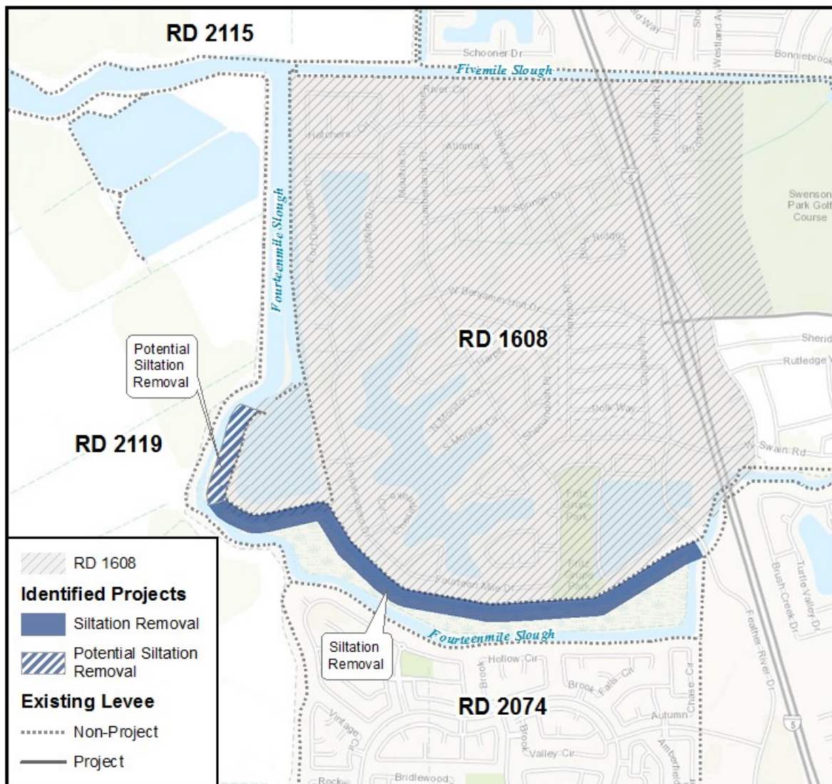
Figure 22 – RD 1608 Sediment Removal Project
