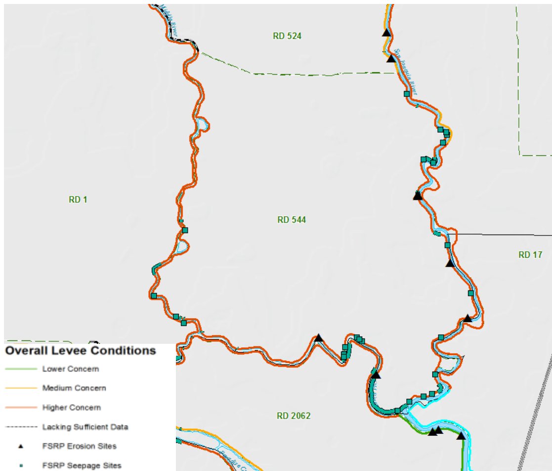
Figure 40 - CVFPP Overall Levee Conditions RD 544
