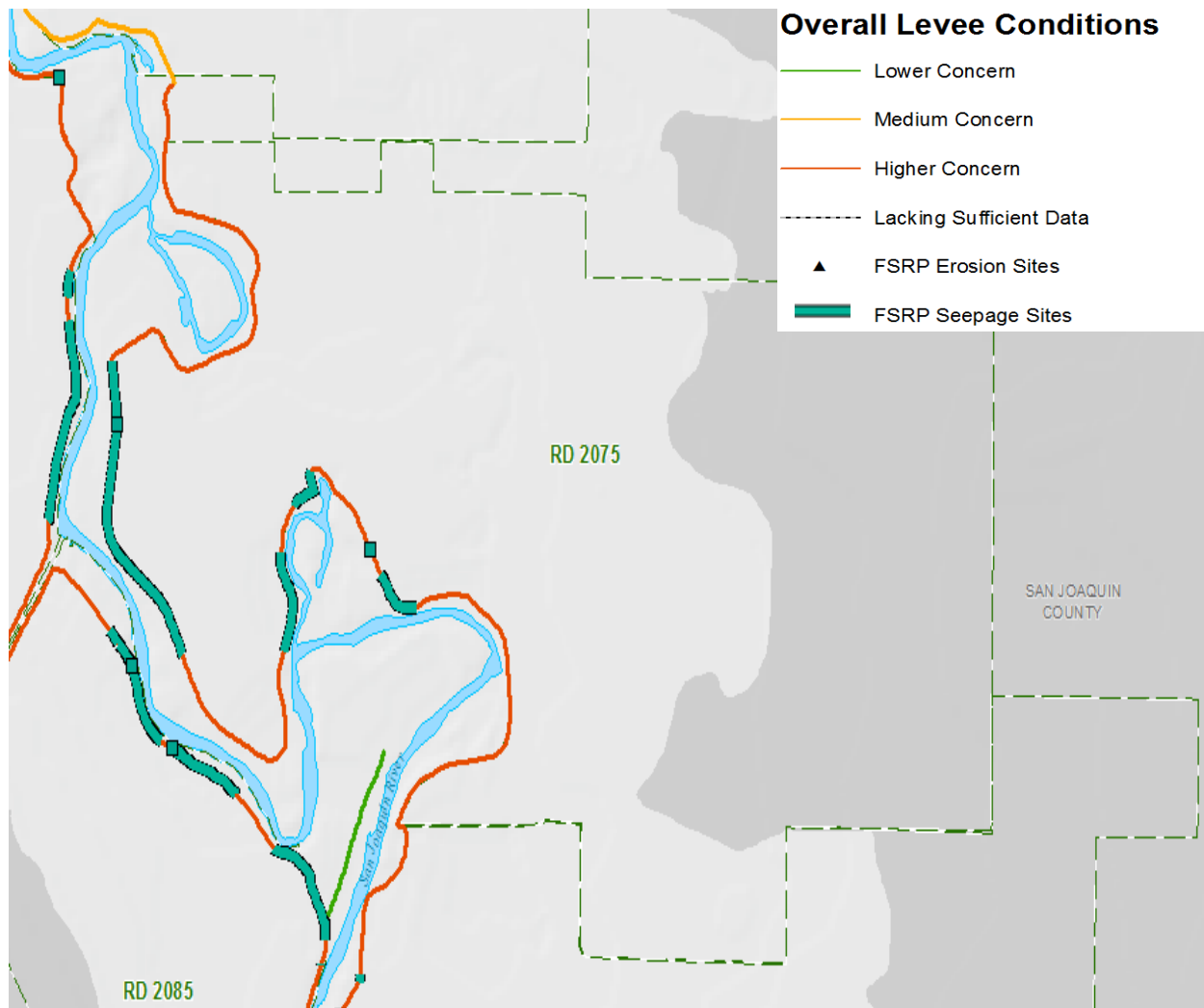
Figure 28 - CVFPP Overall Levee Conditions RD 2075
