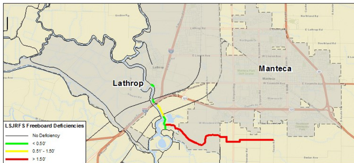
Figure 10 - RD 17 Freeboard Deficiencies
