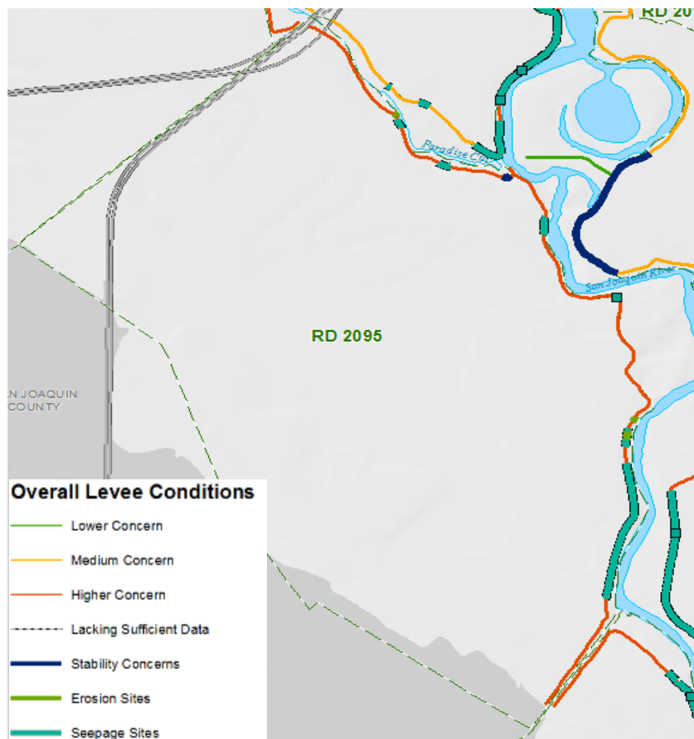
Figure 52 - CVFPP Overall Levee Conditions RD 2095
