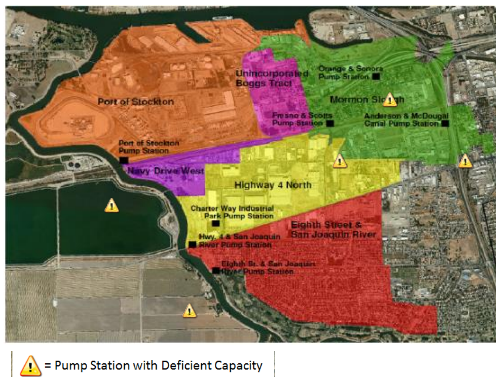
Figure 20 – RD 404 Interior Drainage
